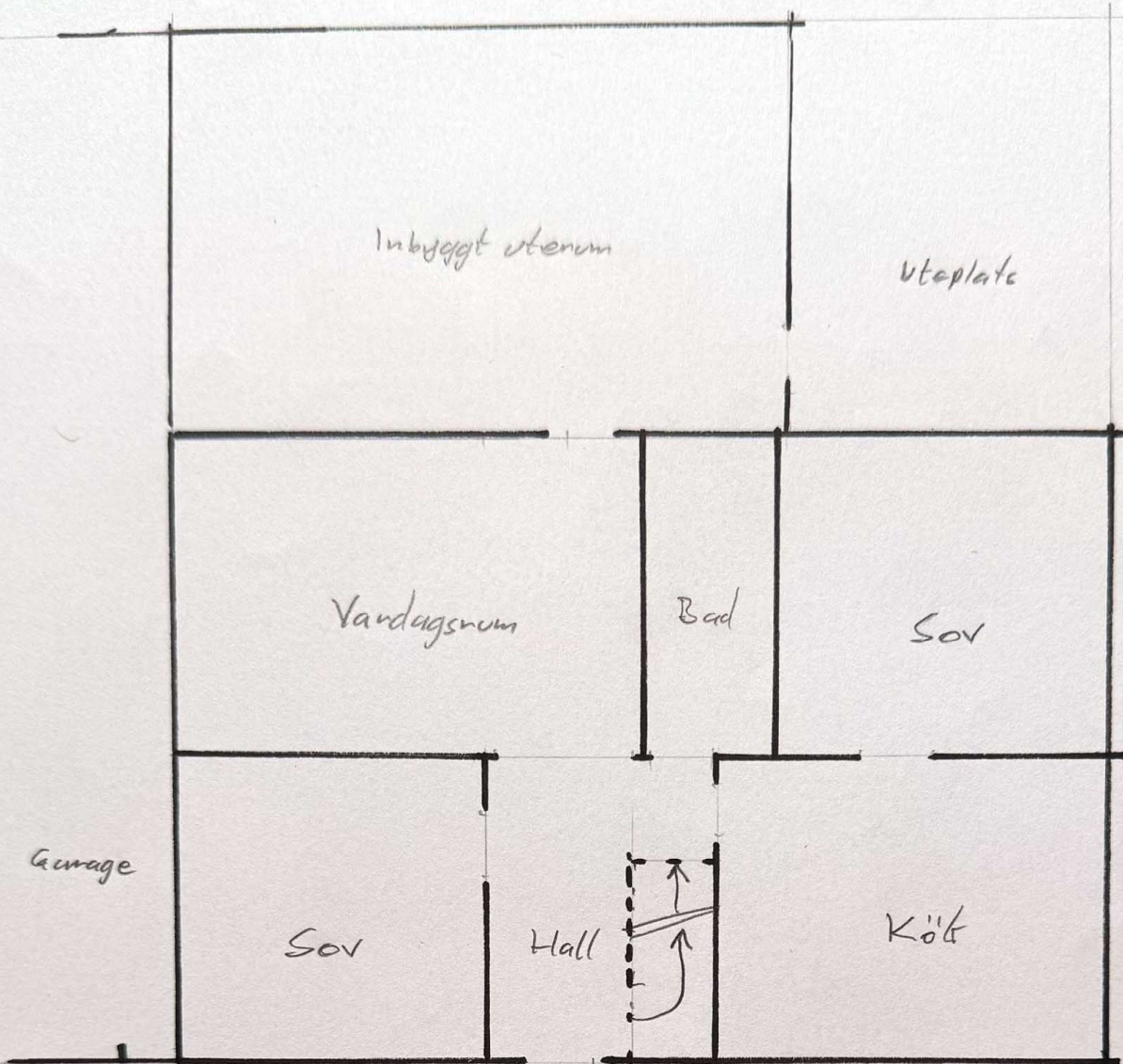
Bottenplan
